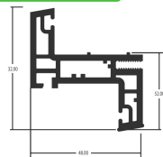
7000 Frame / Vent
