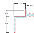
7501 Aluminium Internal Fixing Profile
